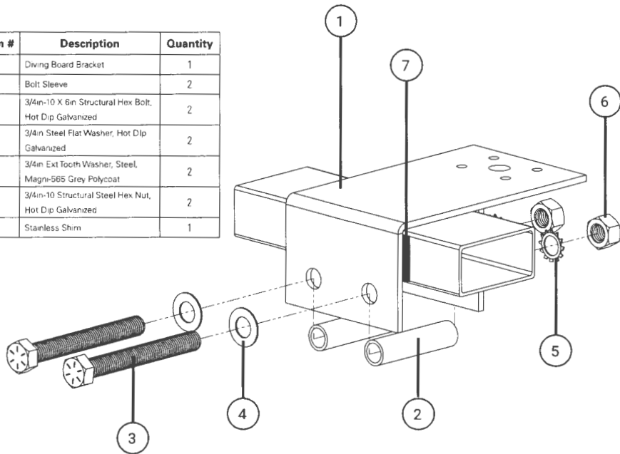
DB2 Diving Board Kit Parts Diagram
