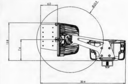
3c Yoke Mount with Visor (VHE, CV1, CV2, CV5)
