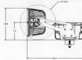
3a Yoke Mount
