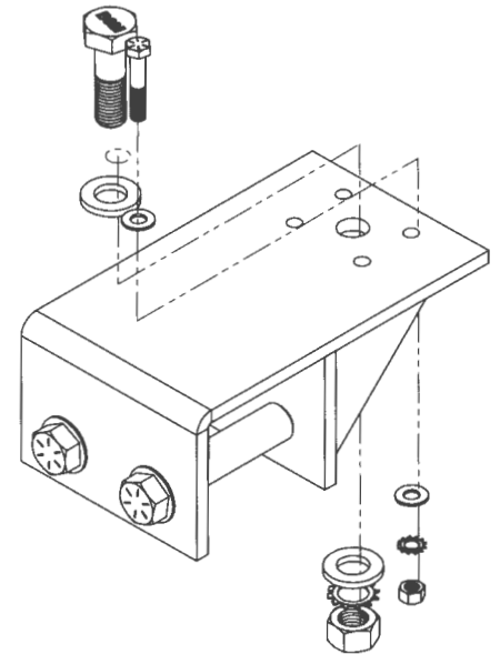
DB3 Diving Board Kit (DVGBRD) with Additional (HRDM34) Mounting Fastener Hardware Kit
