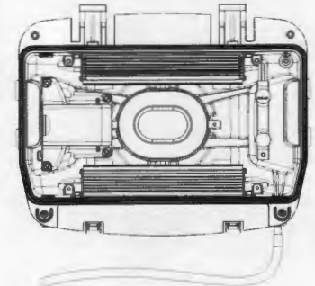
6b Closed Driver Box in Local Yoke Mount Configuration
