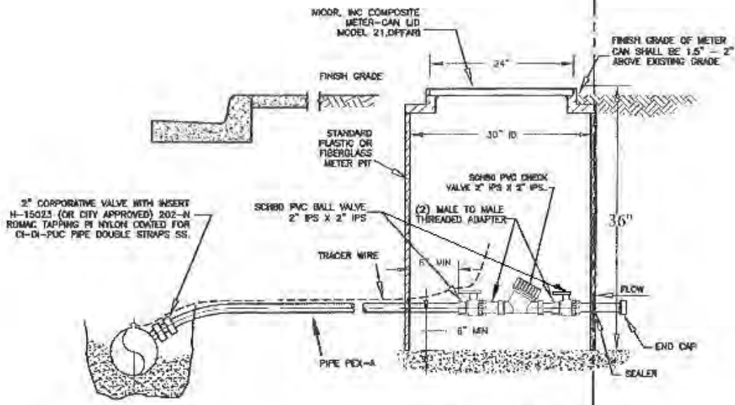
SECTION VIEW
