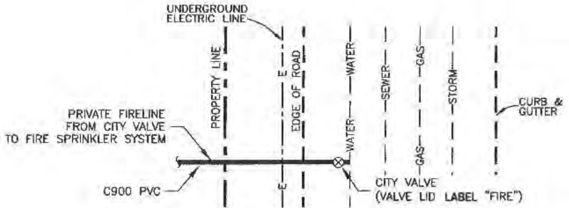
DEDICATED FIRE LINE (TYPICAL)
