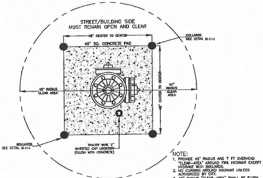
DOUBLE STEAMER TOP VIEW
